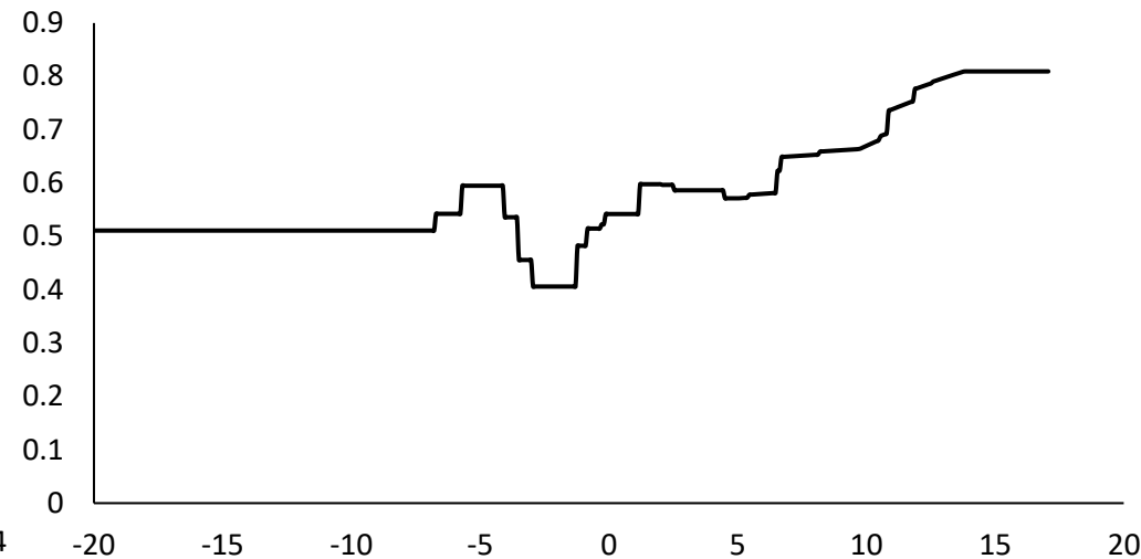
Mean temperature of coldest quarter
