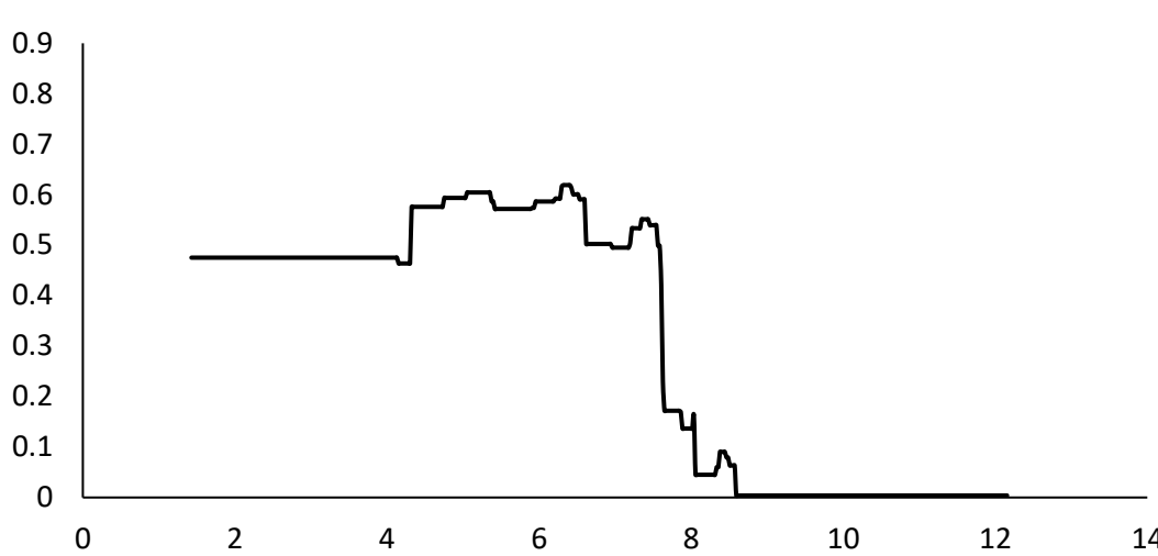
Temperature seasonality
