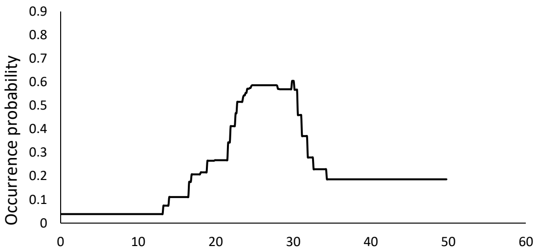
Maximum temperature of warmest month
