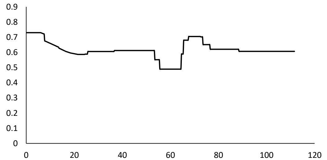
Precipitation seasonality
