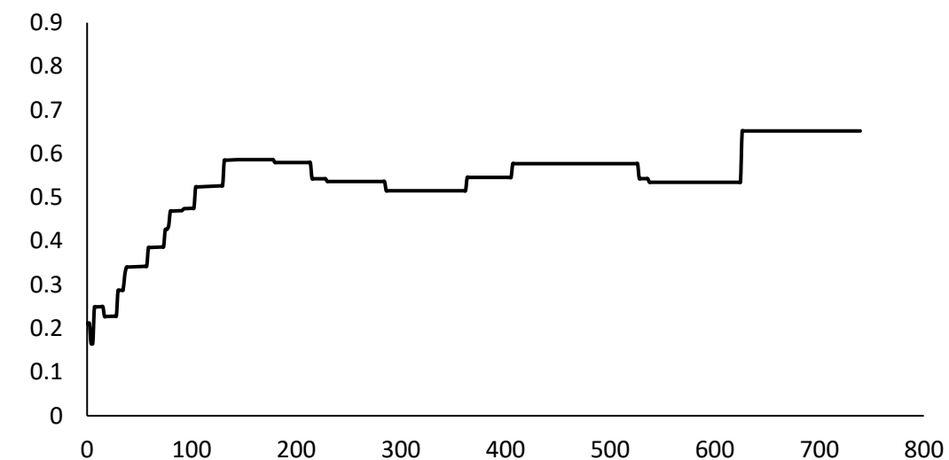
Precipitation of warmest quarter
