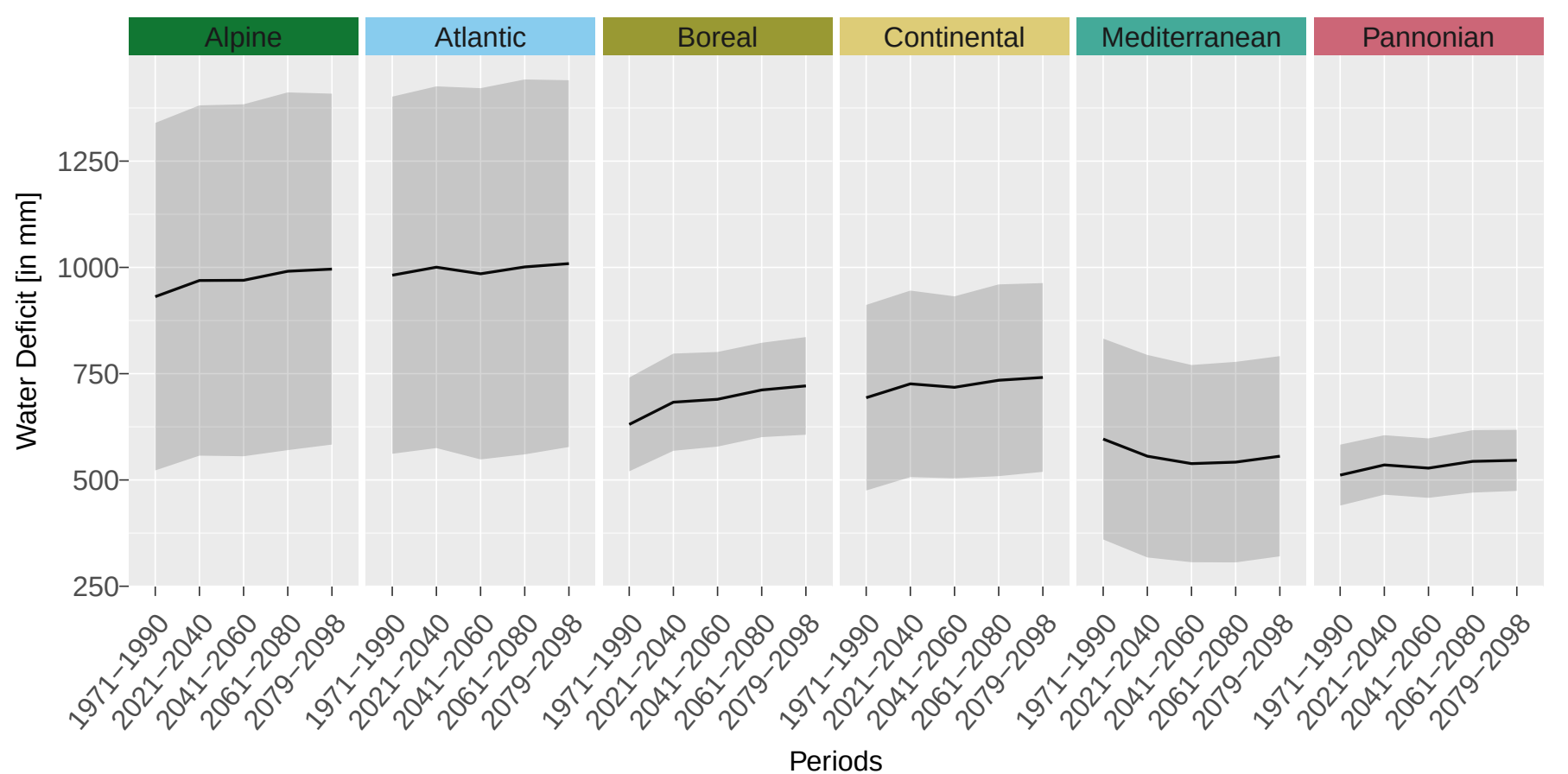
(c) Water Deficit
