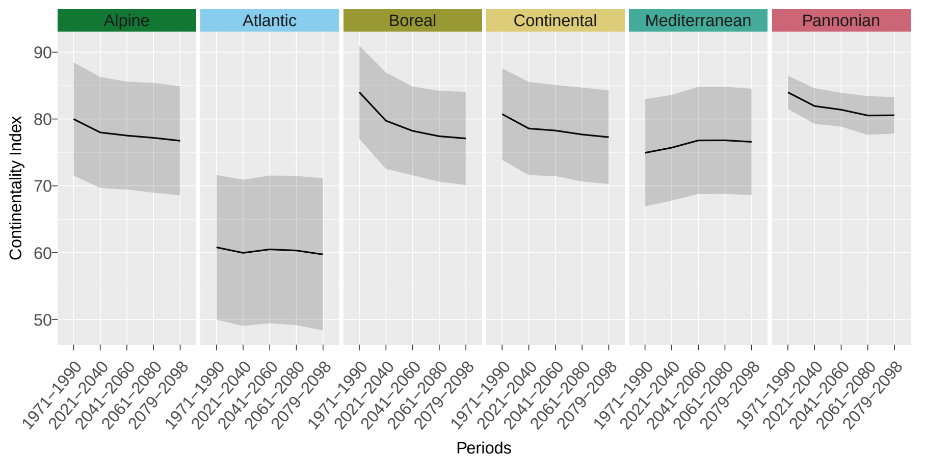
(b) Continuity Index
