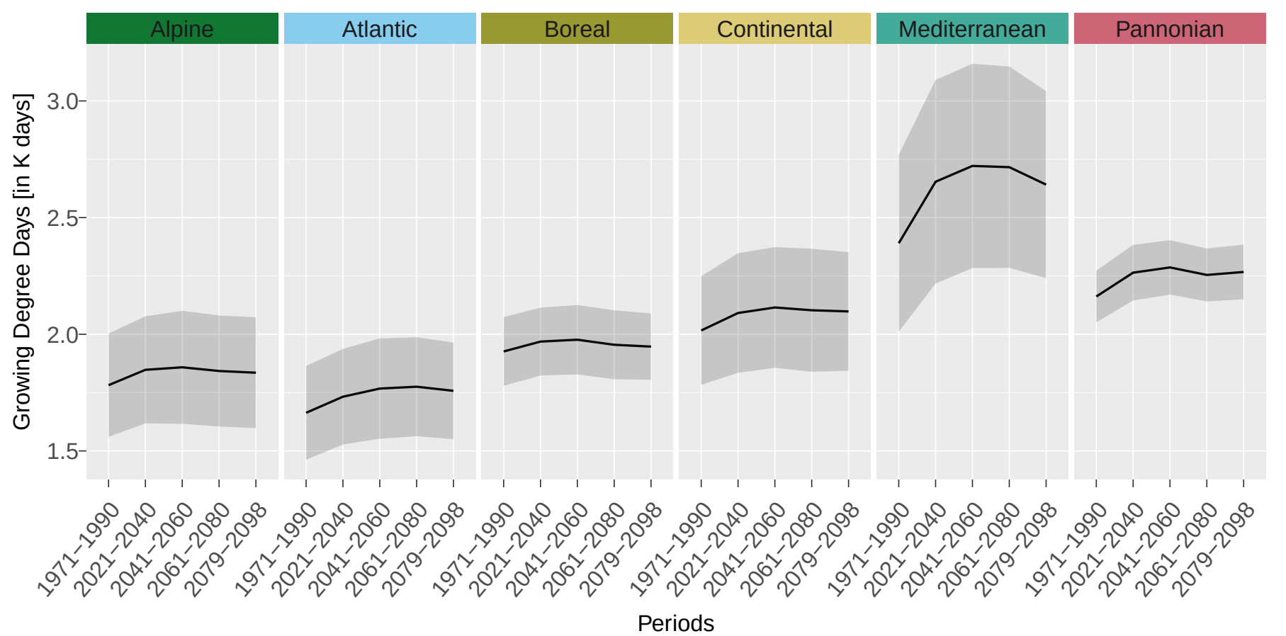
(a) Growing Degree Days
